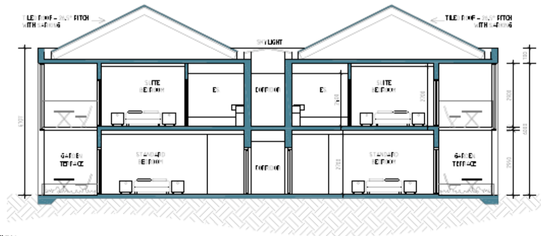
TYPICAL SECTION STANDARD ROOM & SUITE
