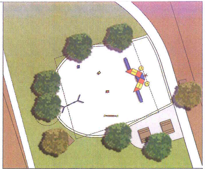
DETAIL PLAN OF PLAYGROUND AND SEATING AREA SCALE 1:200 AT A2
