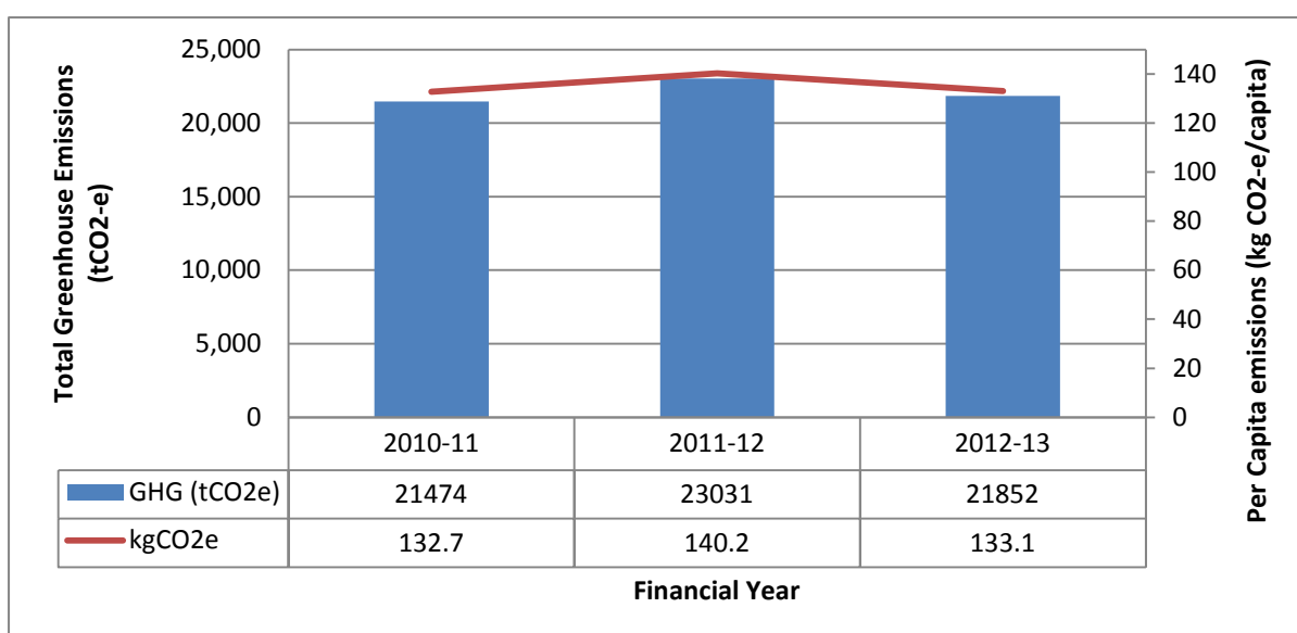
Figure 12: City of Joondalup total annual Corporate greenhouse gas emissions and per capita emissions since 2010/11
