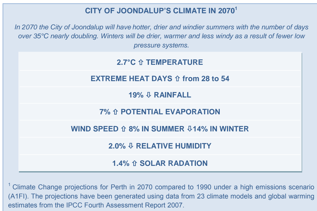
Figure 19: Climate Change Scenario for the City of Joondalup in 2070 56
