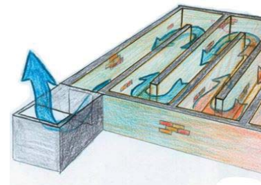
THERMAL LABYRINTH DIAGRAM
